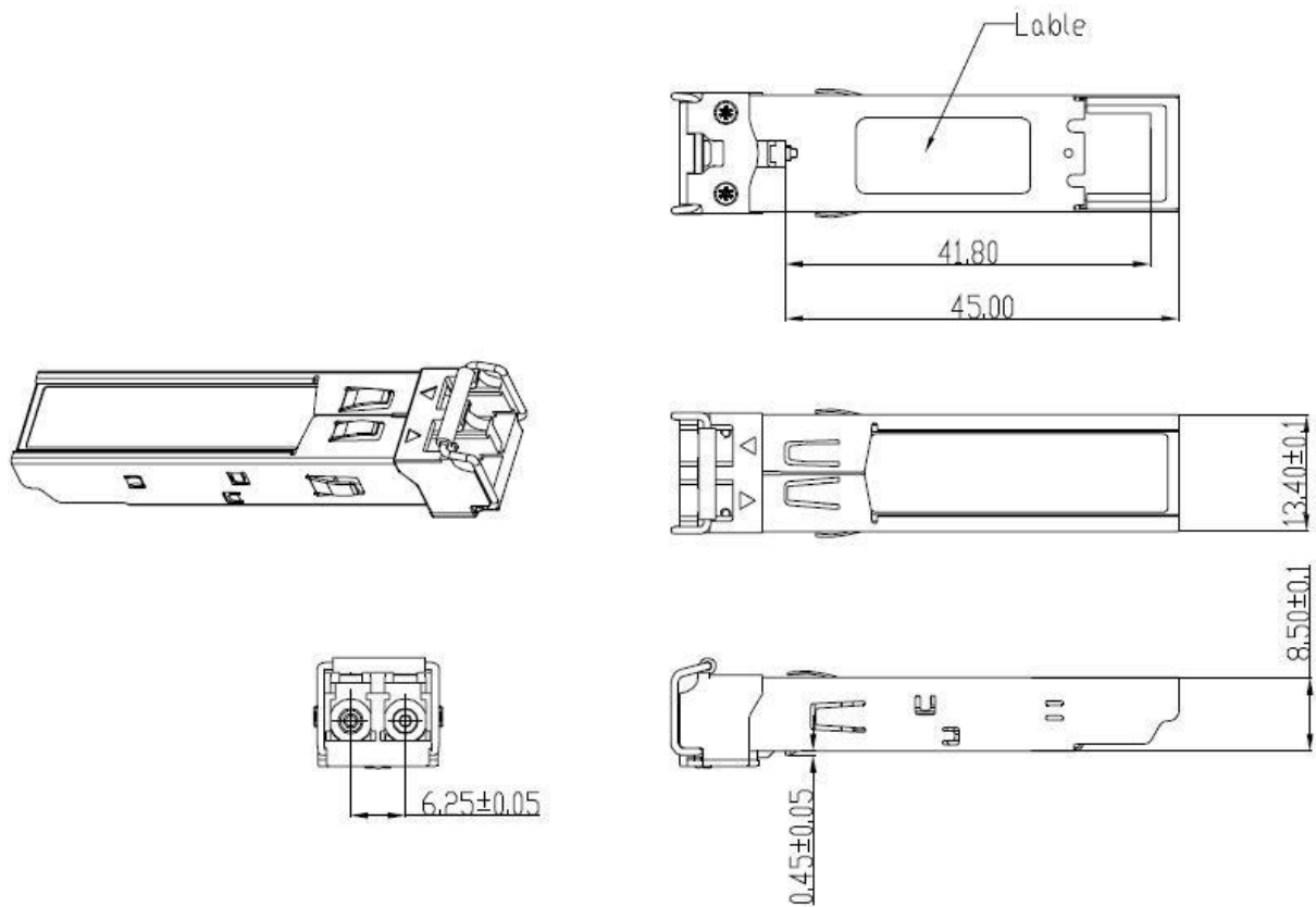
Figure4. Mechanical Specifications
