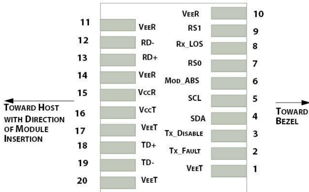
Figure1.Electrical Pin-out Details
