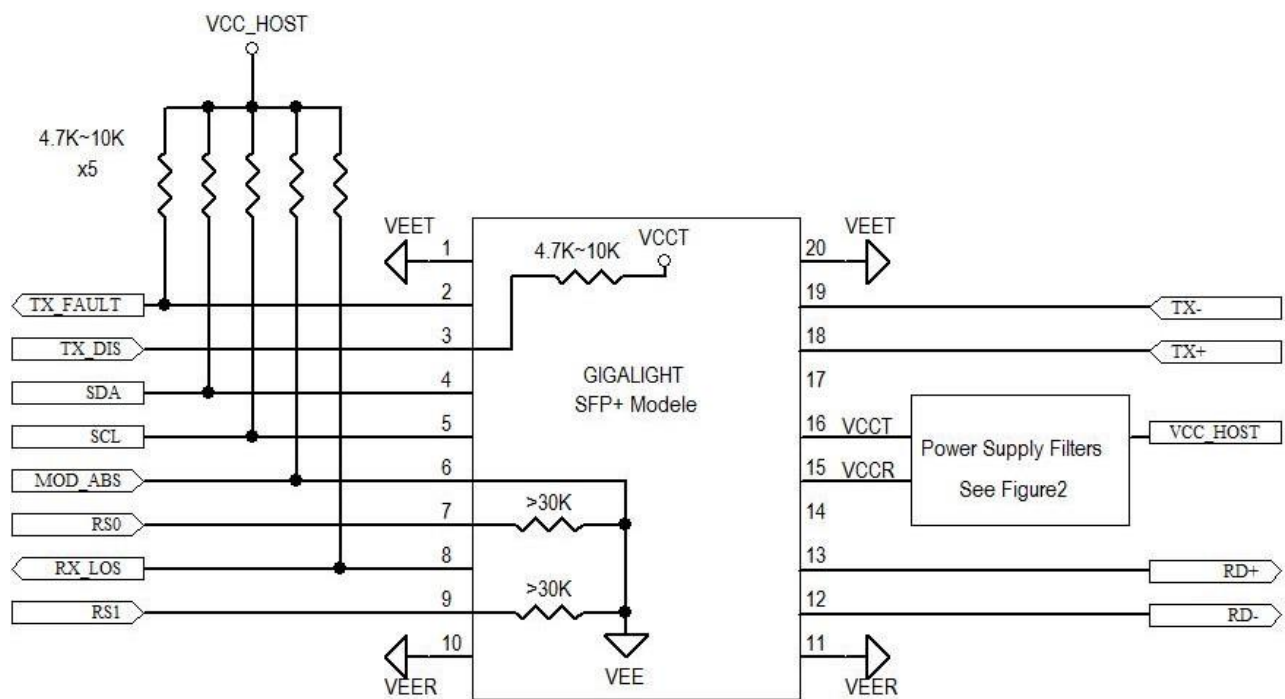
Figure3. Host-Module Interface
