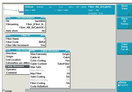
Figure 3. Advanced cable information for metro network
